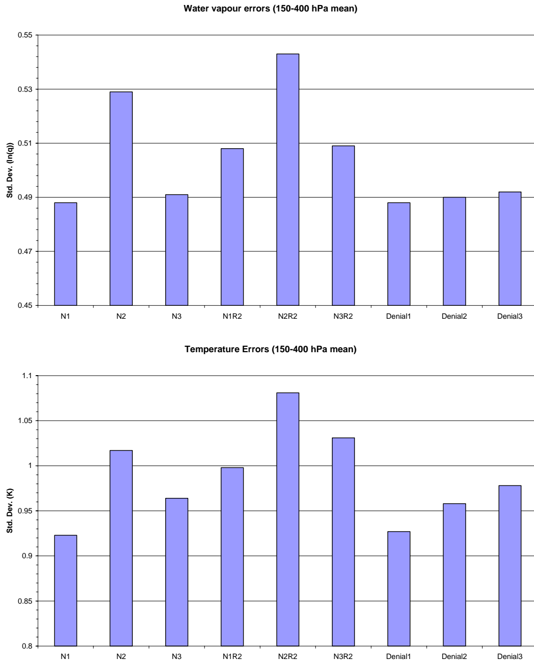
Figure 11: Mean errors between 150 and 400 hPa in water vapour and temperature retrievals for all the 1D-Var runs described in this study. N1, N2 and N3 refer to the “best”, “worst”, and “compromise” noise scenarios respectively. R1 and R2 refer to full AIRS resolution and half AIRS resolution.
