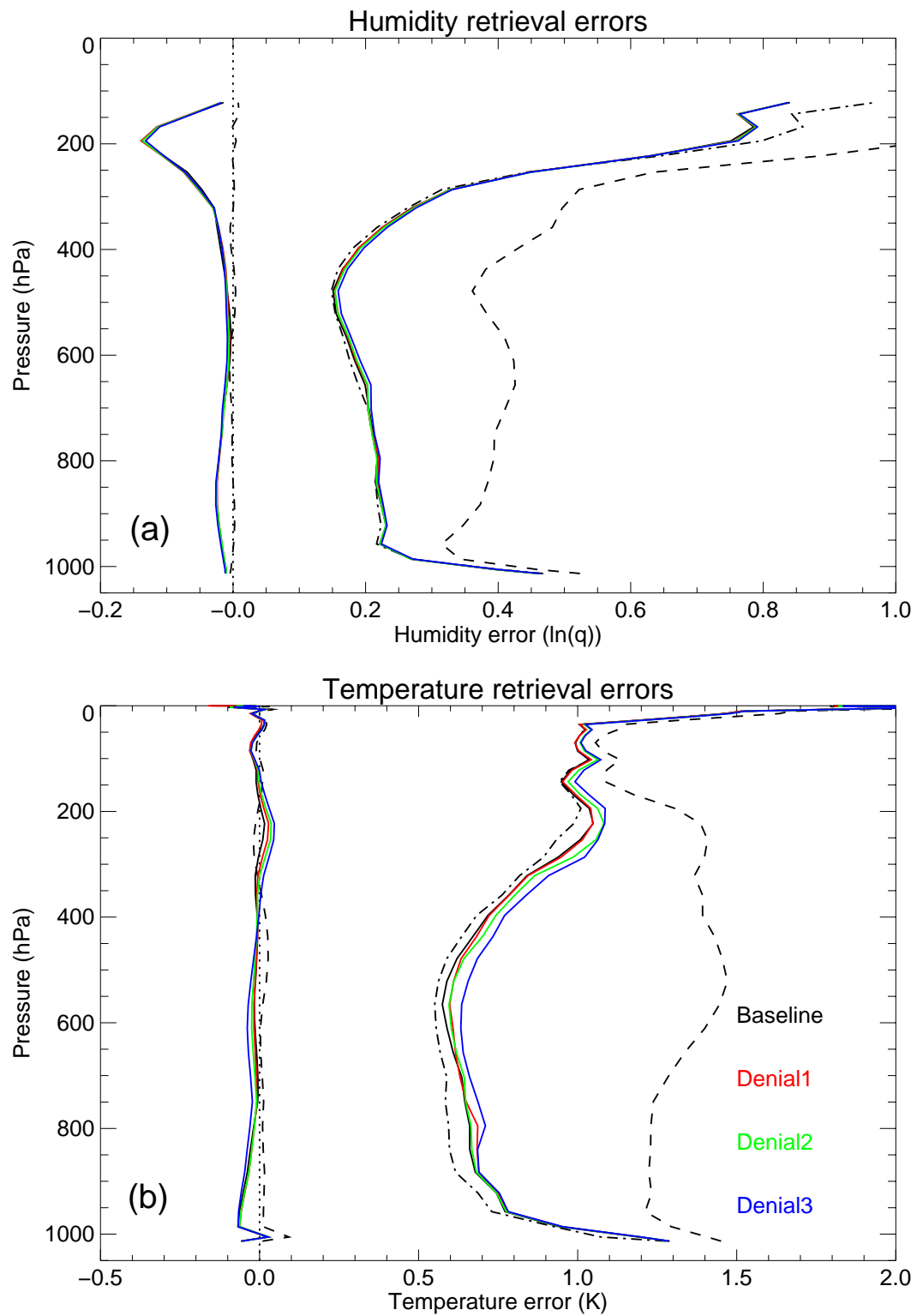
Figure 9: As Figure 4, but showing retrieval errors for the three CO 2 band data denial experiments for the N1 (best) noise case.
