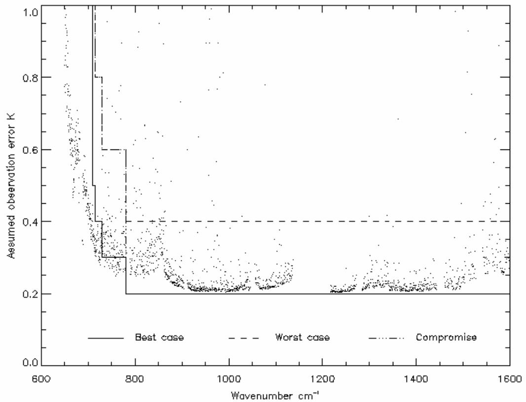
Figure 3: Measurement errors simulated in this study (at 280K scene temperature), compared with AIRS errors (dots). Solid line: best case (N1); Dashed line: worst case (N2); Dot-dashed line: compromise case (N3).
