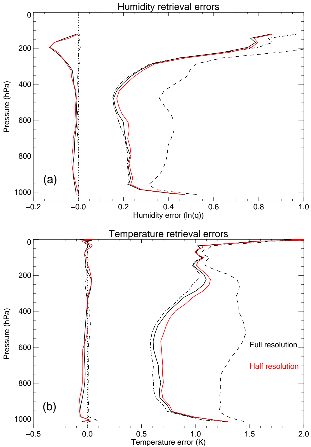
Figure 8: As Figure 4, but showing retrieval errors for full AIRS resolution (black) and half AIRS resolution (red), for the N3 (compromise) noise case. The dot-dashed line shows the linear analysis error expected for the N3 noise case with full resolution.
