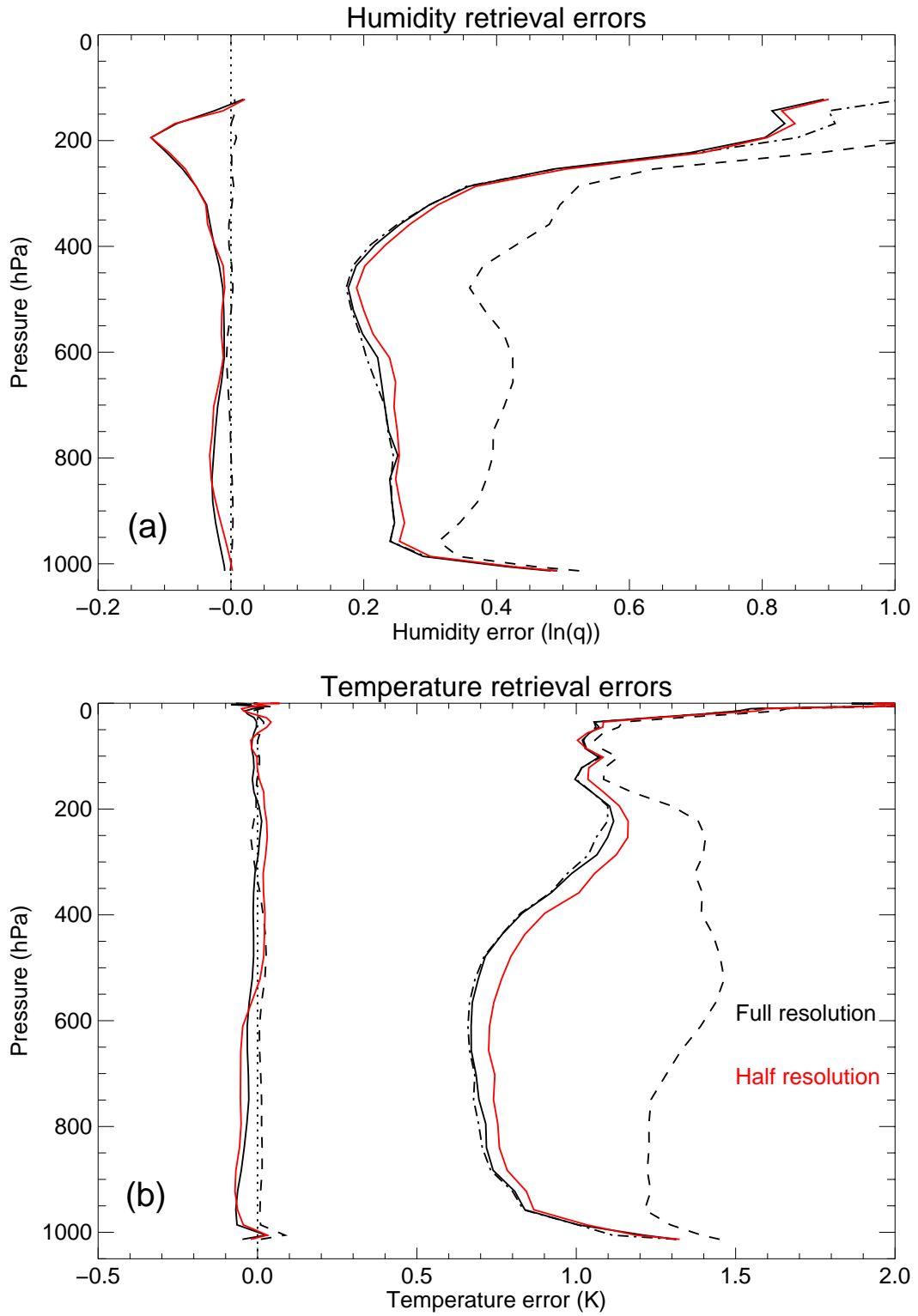
Figure 7: As Figure 4, but showing retrieval errors for full AIRS resolution (black) and half AIRS resolution (red), for the N2 (worst) noise case. The dot-dashed line shows the linear analysis error expected for the N2 noise case with full resolution.
