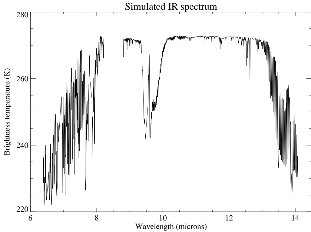
Figure 2: Example infrared spectrum as simulated for the 1D-Var study.
