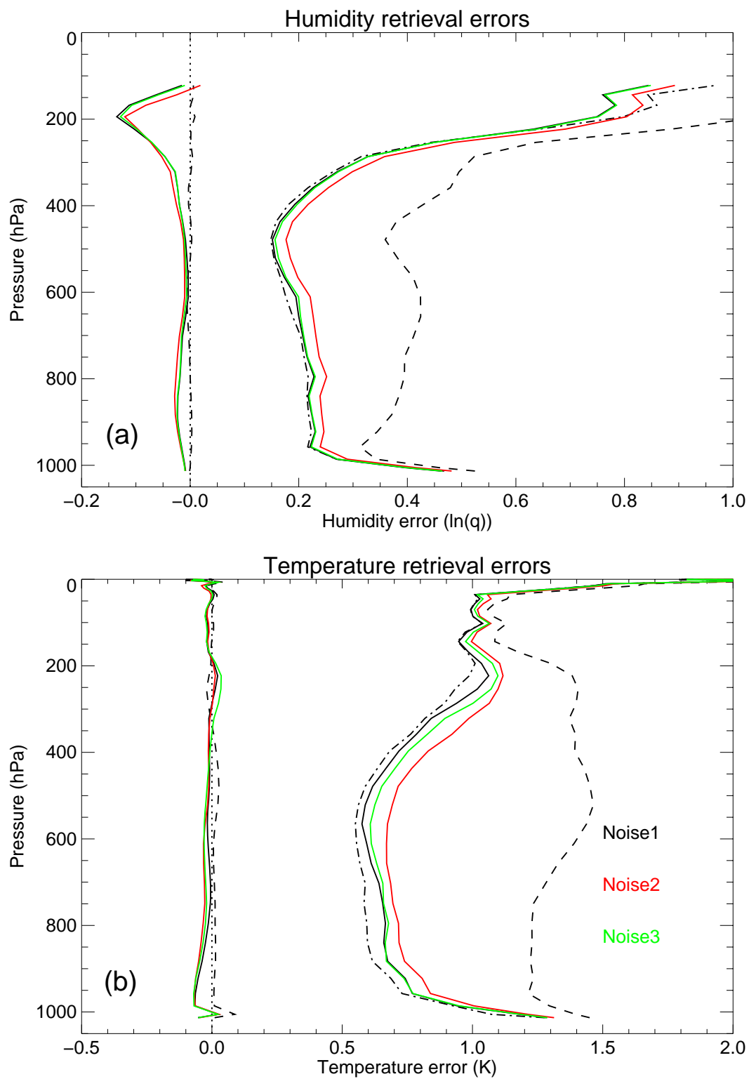
Figure 4: Retrieval errors for three noise scenarios. Left: bias; Right: standard deviation. Solid lines: retrievals; dashed lines: background; dot-dashed line: linear analysis error for N1 (best) noise case.
