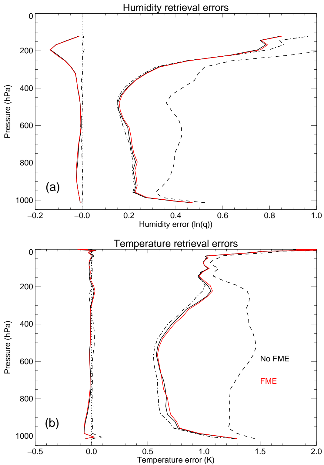
Figure 5: As Figure 4, but showing the effect of introducing a forward model error of 0.2 K (for the best (N1) noise case).
