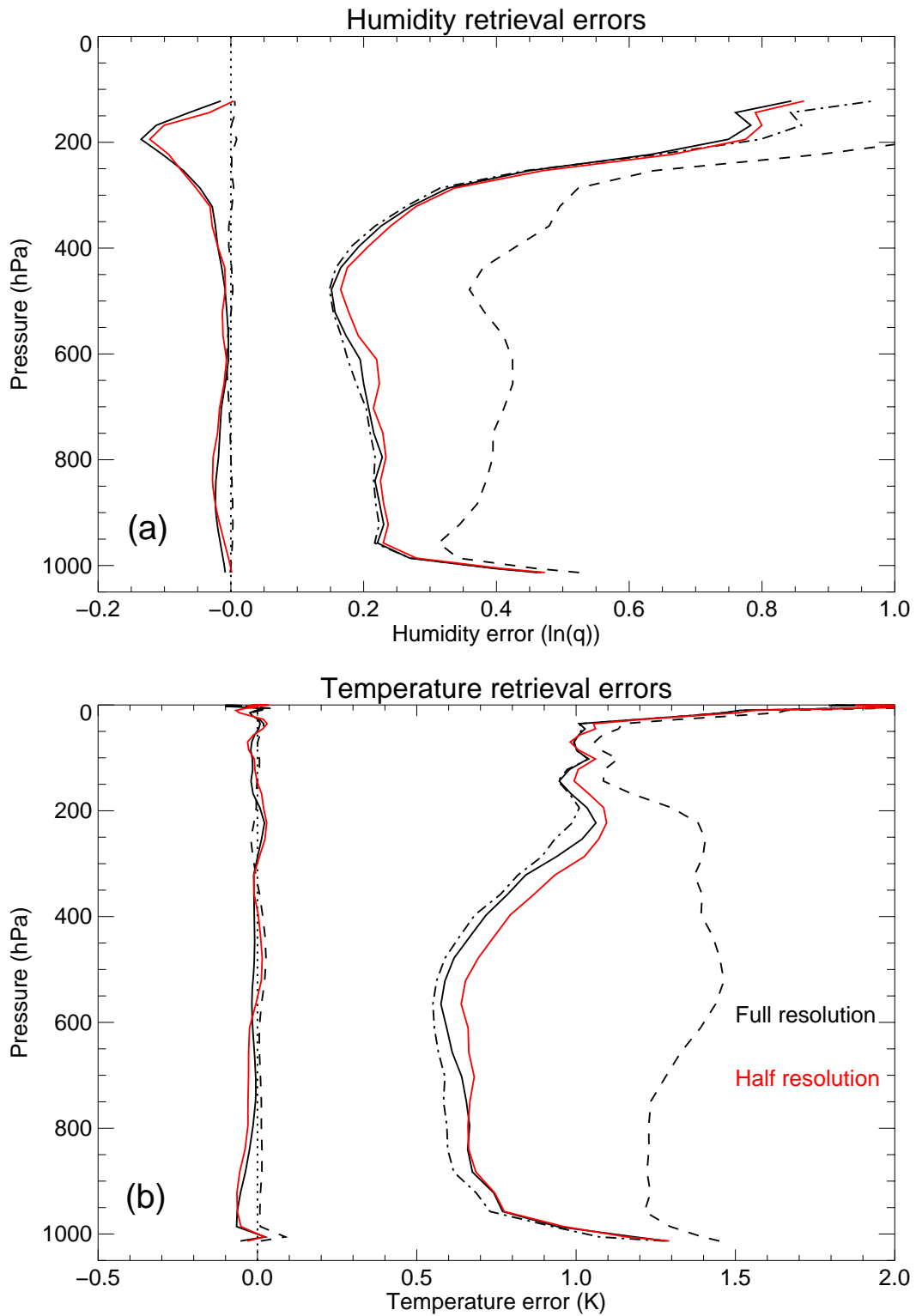
Figure 6: As Figure 4, but showing retrieval errors for full AIRS resolution (black) and half AIRS resolution (red), for the N1 (best) noise case. The dot-dashed line shows the linear analysis error expected for the N1 noise case with full resolution.
