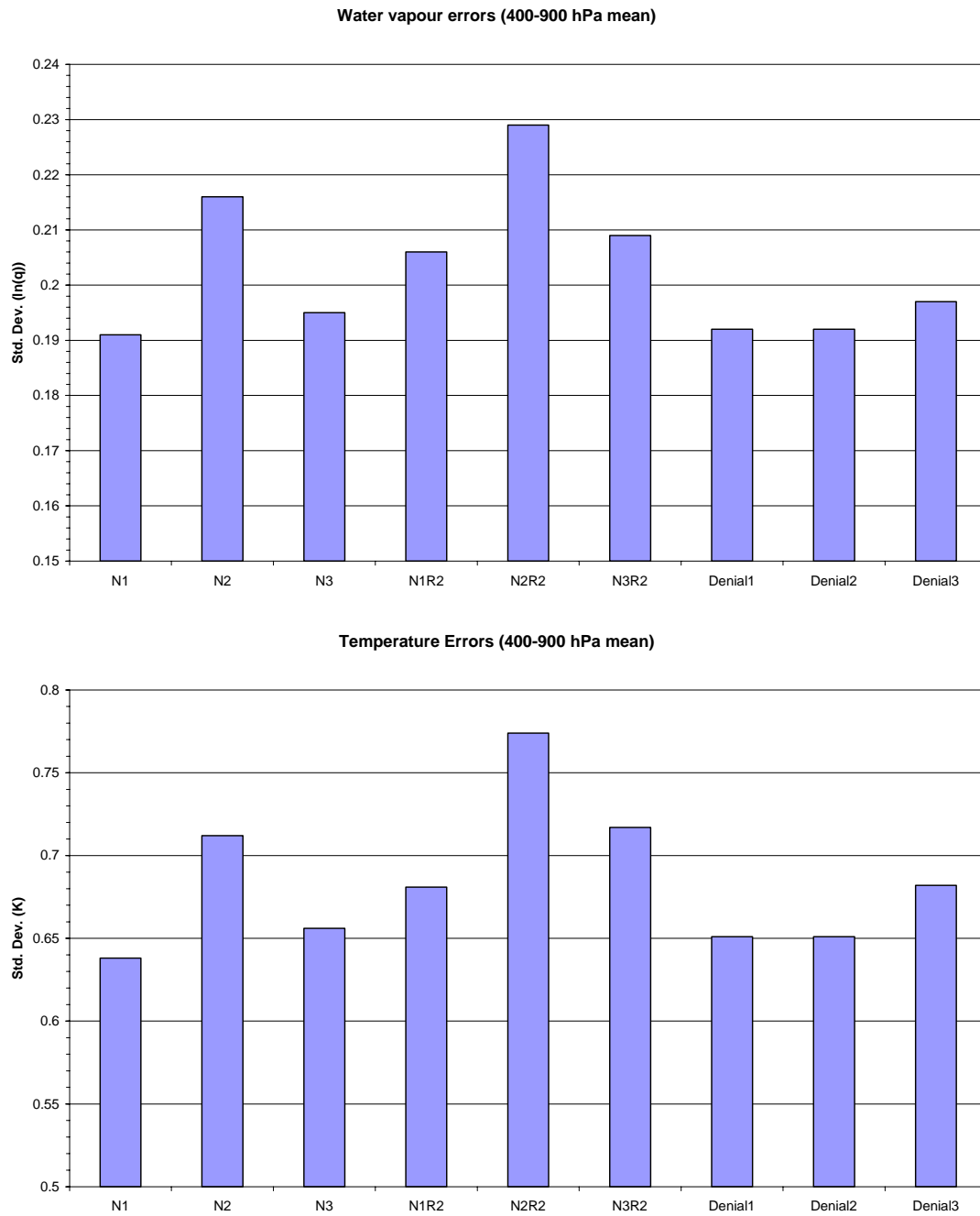
Figure 10: Mean errors between 400 and 900 hPa in water vapour and temperature retrievals for all the 1D-Var runs described in this study. N1, N2 and N3 refer to the “best”, “worst”, and “compromise” noise scenarios respectively. R1 and R2 refer to full AIRS resolution and half AIRS resolution.
