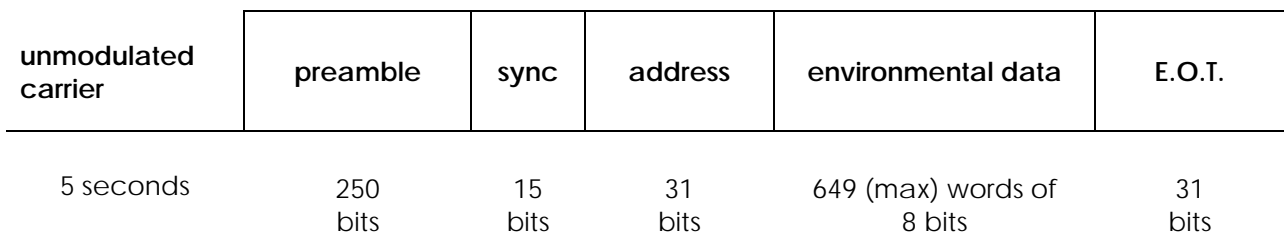
Figure 2.1 Report Format
