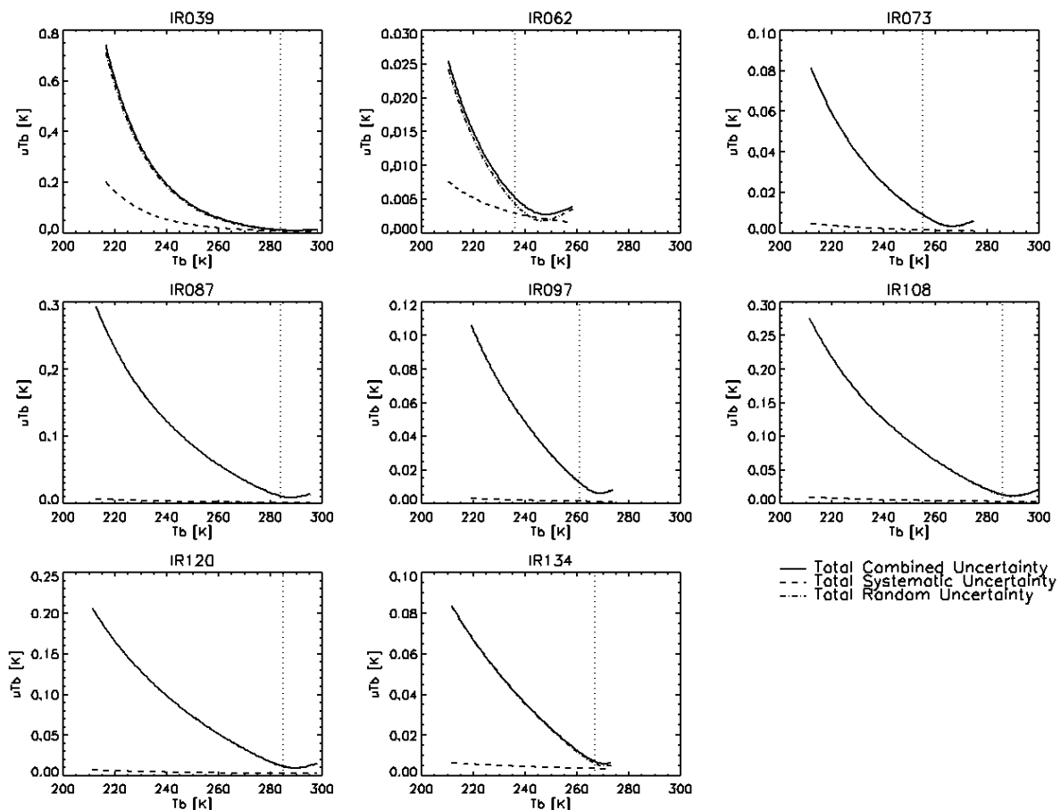
Figure 5 – Impact of Total Systematic and Random Errors on Uncertainty of the Brightness Temperatures ( T_b ) produced by the GSICS Correction for a range of scene radiances for each infrared channel of Meteosat9/SEVIRI using MetopA/IASI reference. Dotted vertical line shows standard scene radiance for each channel.
