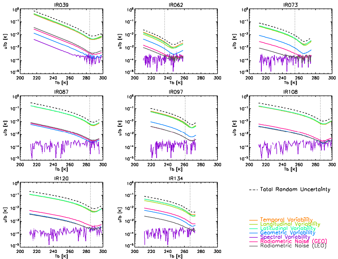
Figure 4 – Contribution of each source of Random Error to the Uncertainty of the Brightness Temperatures ( T_b ) produced by the GSICS Correction for a range of scene radiances for each infrared channel of Meteosat9/SEVIRI using MetopA/IASI reference. Dotted vertical line shows standard scene radiance for each channel.
