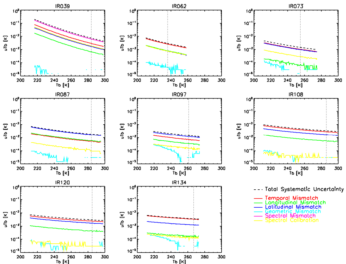
Figure 2 – Contribution of each source of Systematic Error to the Uncertainty of the Brightness Temperatures ( T_b ) produced by the GSICS Correction for a range of scene radiances for each infrared channel of Meteosat9/SEVIRI using MetopA/IASI reference. Dotted vertical line shows standard scene radiance for each channel.
