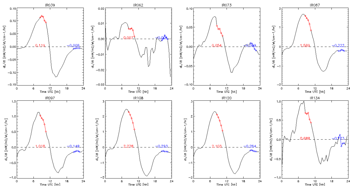
Figure 1 - Time series of mean rate of change of radiances calculated from Meteosat-9 observations on 2009-09-20 over (30^\circ\text{W}-30^\circ\text{E}) \times (30^\circ\text{S}-30^\circ\text{N}) .
